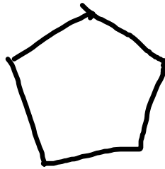
cyclopentane
