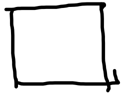
cyclobutane
