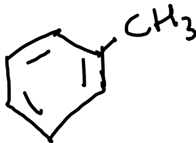
methylbenzene phenylmethane toluene
